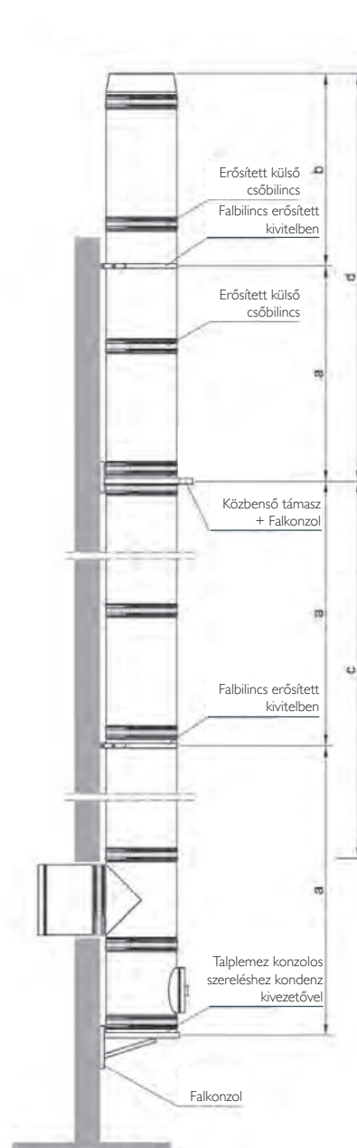
ICS Ø350-700
